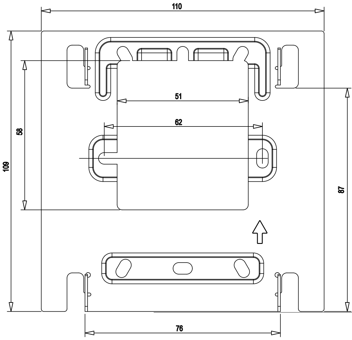
2 FRONT VIEW:WALL MOUNTING BRACKET PLACEMENT
